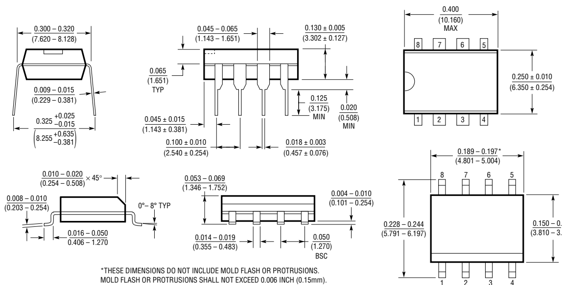
N8 Package 8-Lead Plastic DIP
