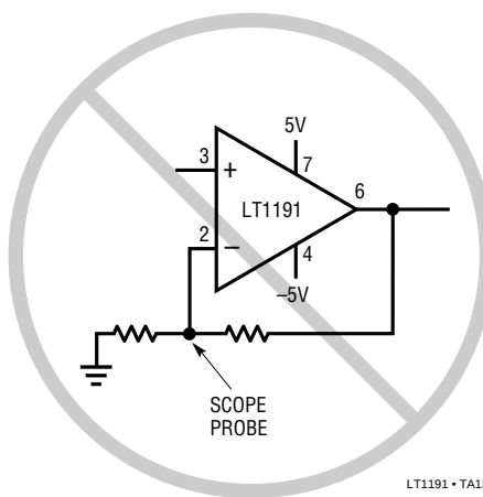
A Scope Probe on the Inverting Input Reduces Phase Margin
