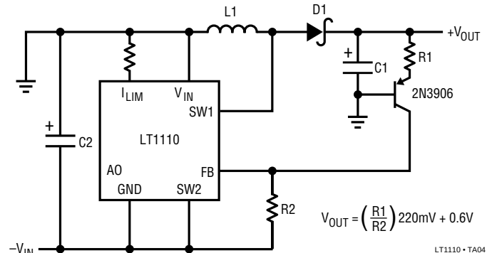
Figure 8. Negative-to-Positive Converter
