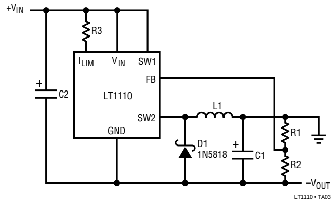
Figure 7. Positive-to-Negative Converter
