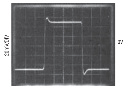
Small-Signal Transient Response V_S = \pm 15V
