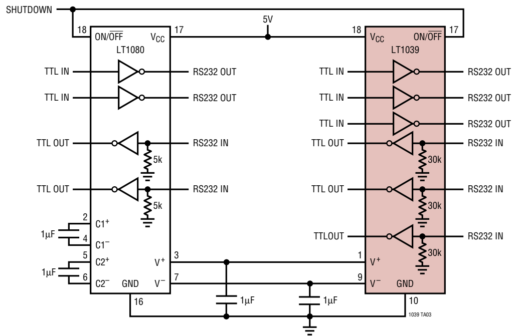
LT1080 (Driver/Receiver with Power Supply) Driving an LT1039
