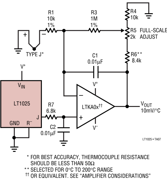
Grounded Thermocouple Amplifier with Positive Output
