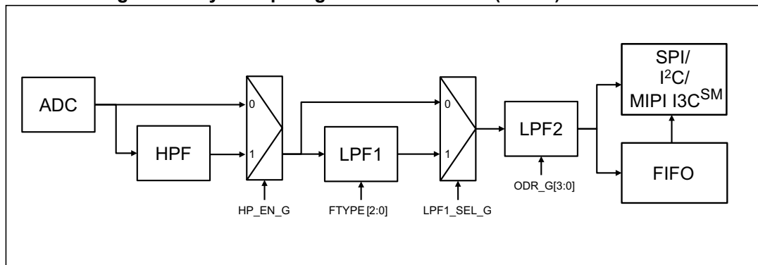
Figure 19. Gyroscope digital chain - Mode 1 (UI/EIS) and Mode 2
