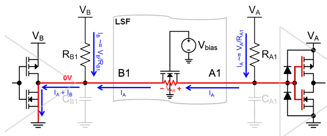
Figure 7. LSF Pass Transistor LOW-State Operation
