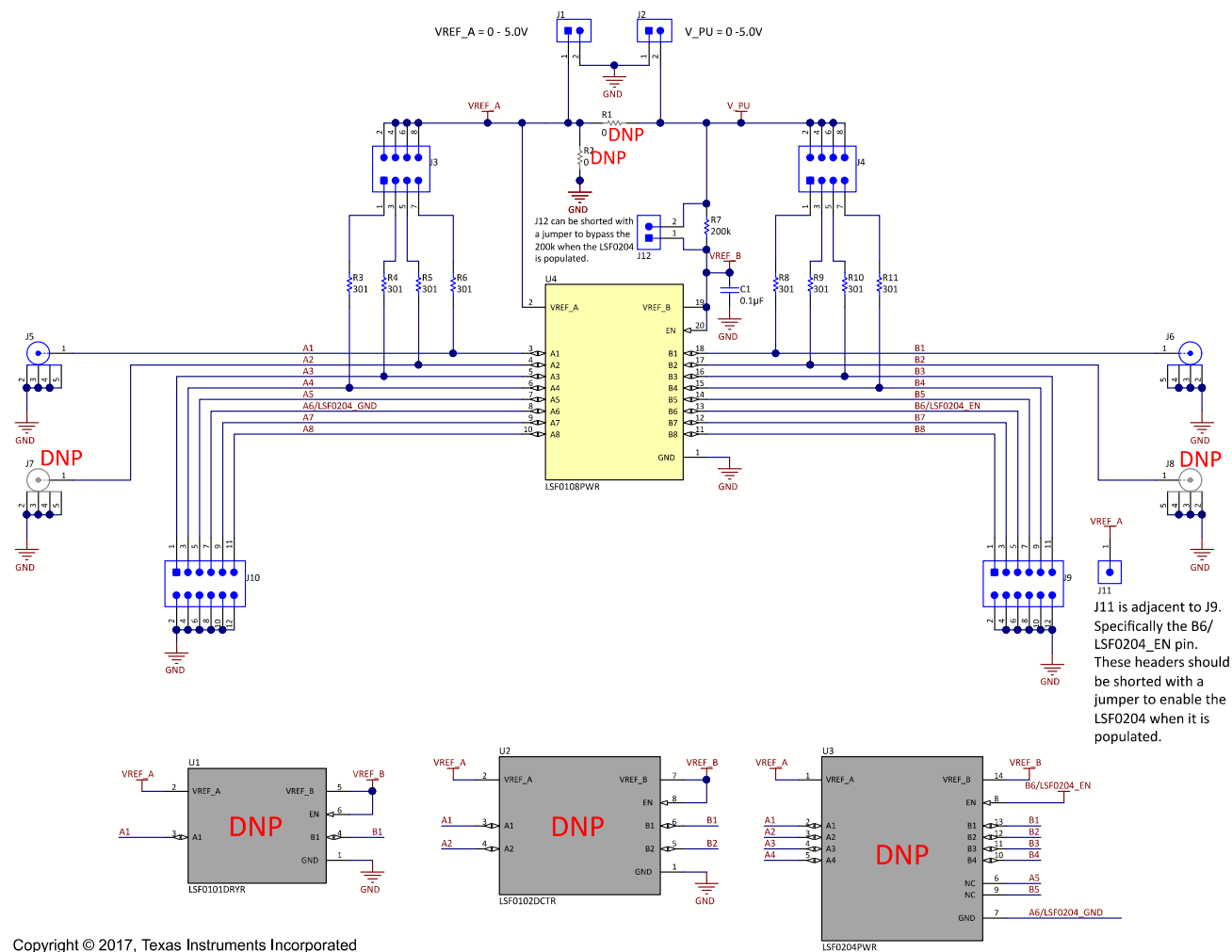
Figure 13. LSF-EVM Schematic (Zoom for Higher Resolution)
