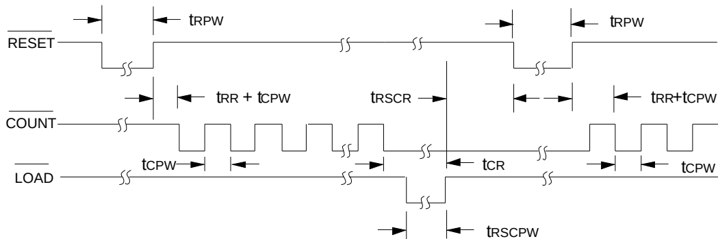
FIGURE 4. COUNTER TIMING DIAGRAM
