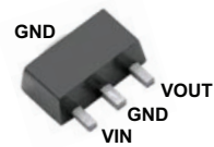
TO-243AA (SOT-89)
