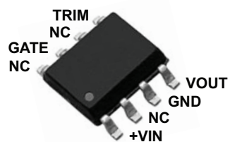
8-Lead SOIC
