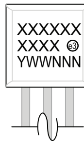
3-lead TO-92
