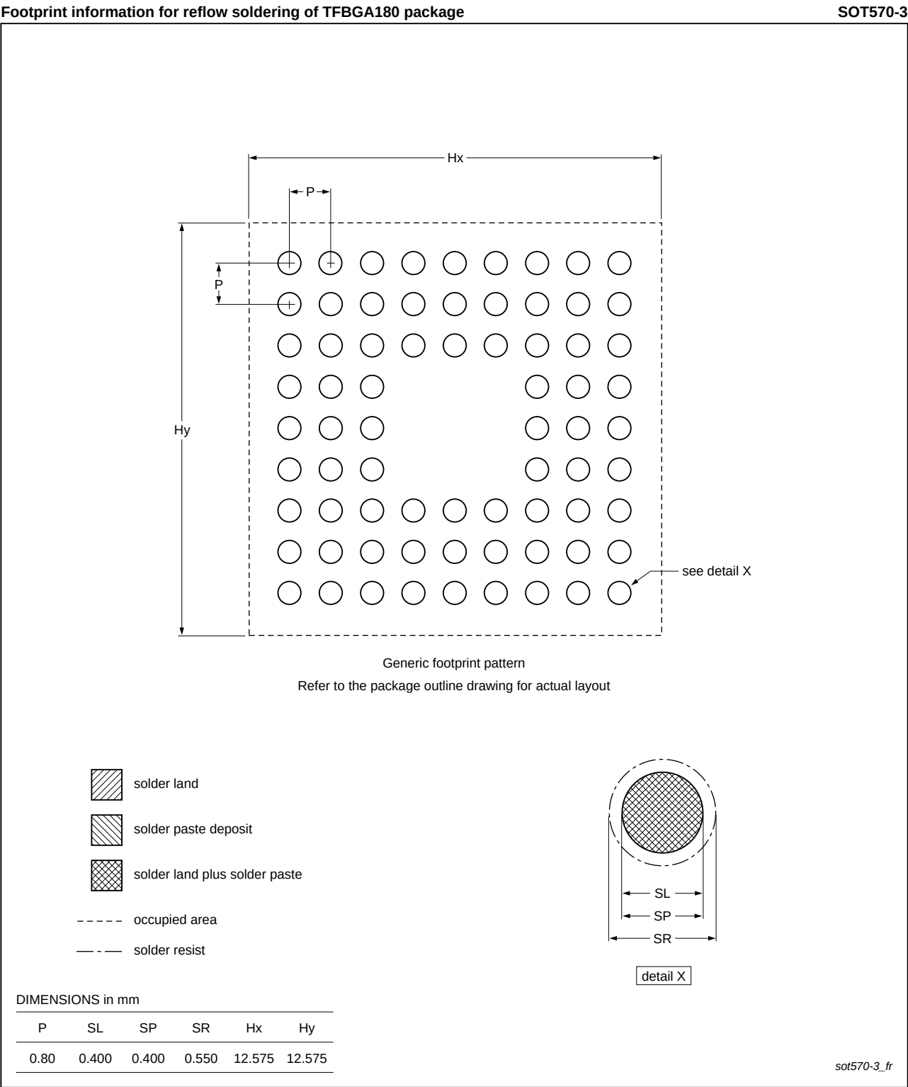
Fig 46. Reflow soldering of the TFBGA180 package
