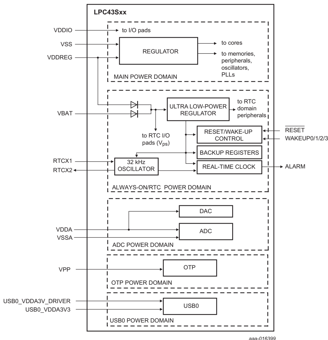
Fig 7. Power domains
