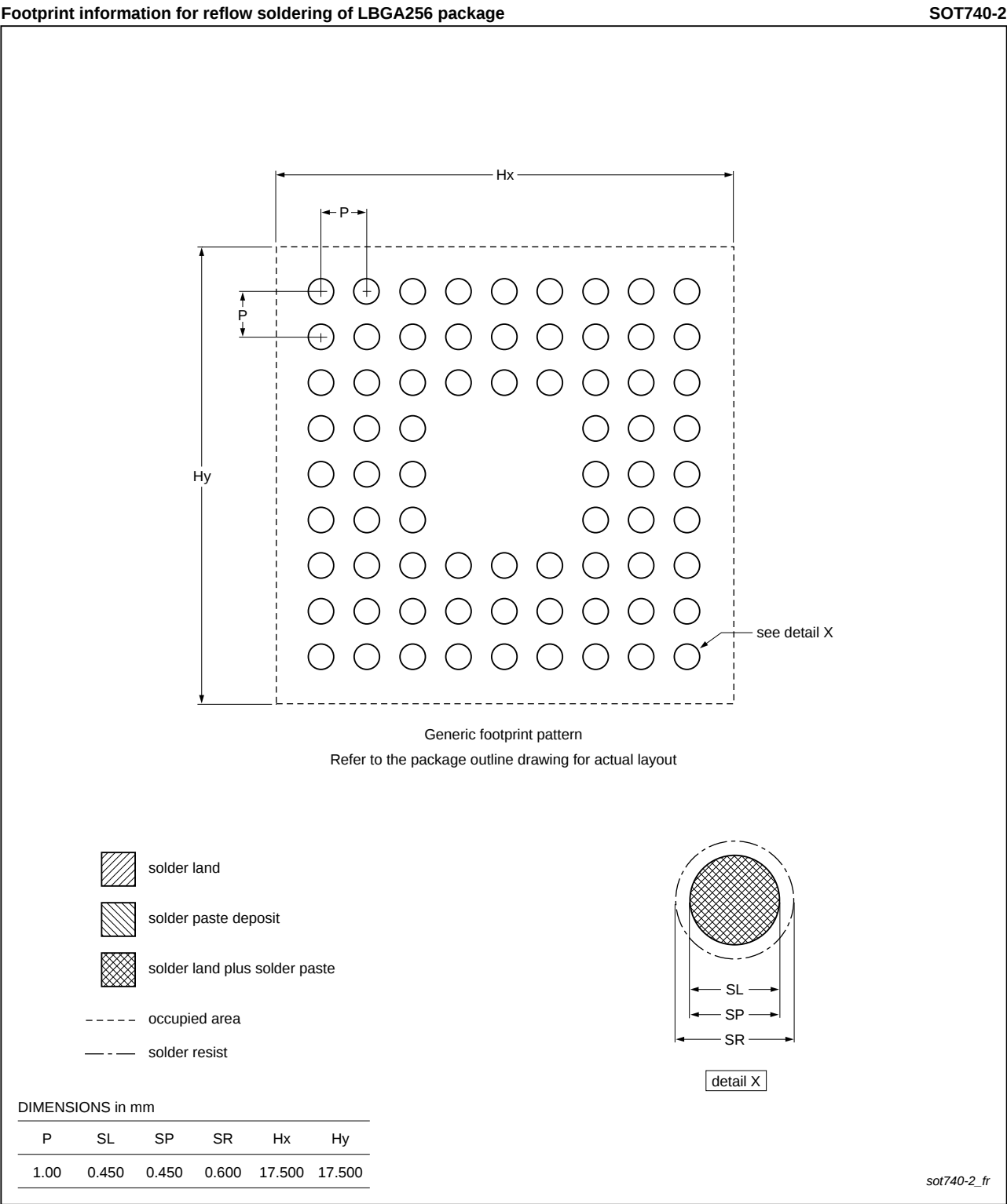
Fig 55. Reflow soldering of the LBG256 package
