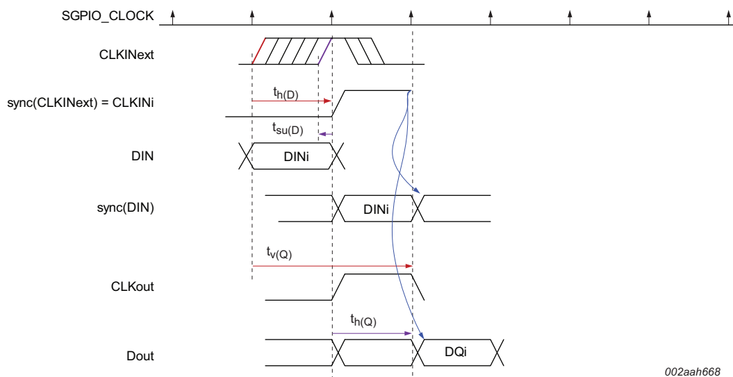
Fig 33. SGPIO timing
