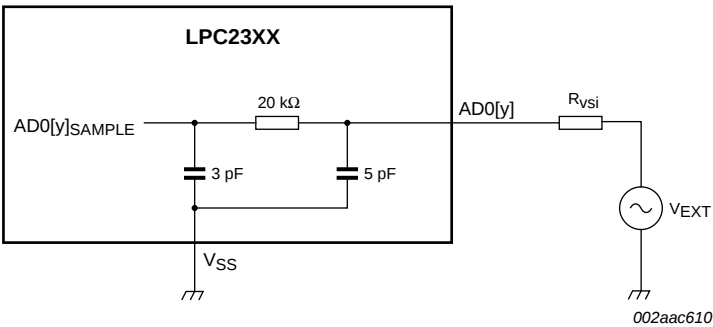
Fig 16. Suggested ADC interface - LPC2361/2362 AD0[y] pin
