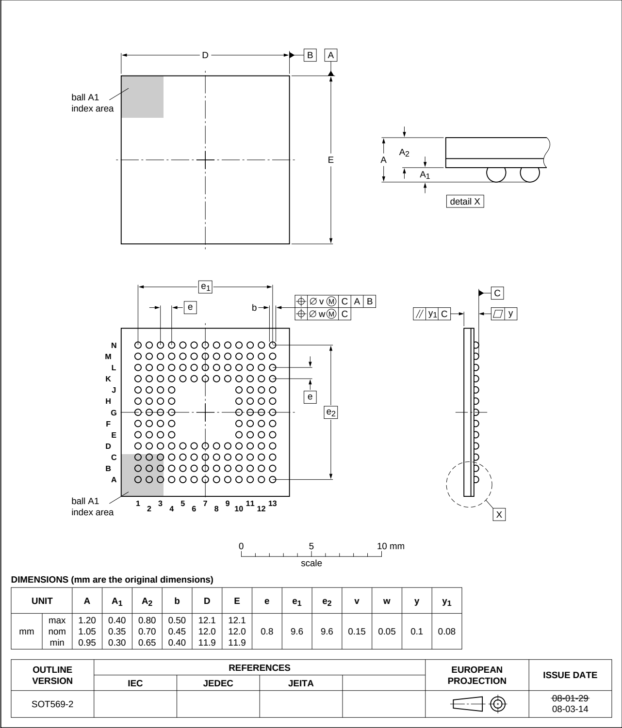
TFBGA144: plastic thin fine-pitch ball grid array package; 144 balls
