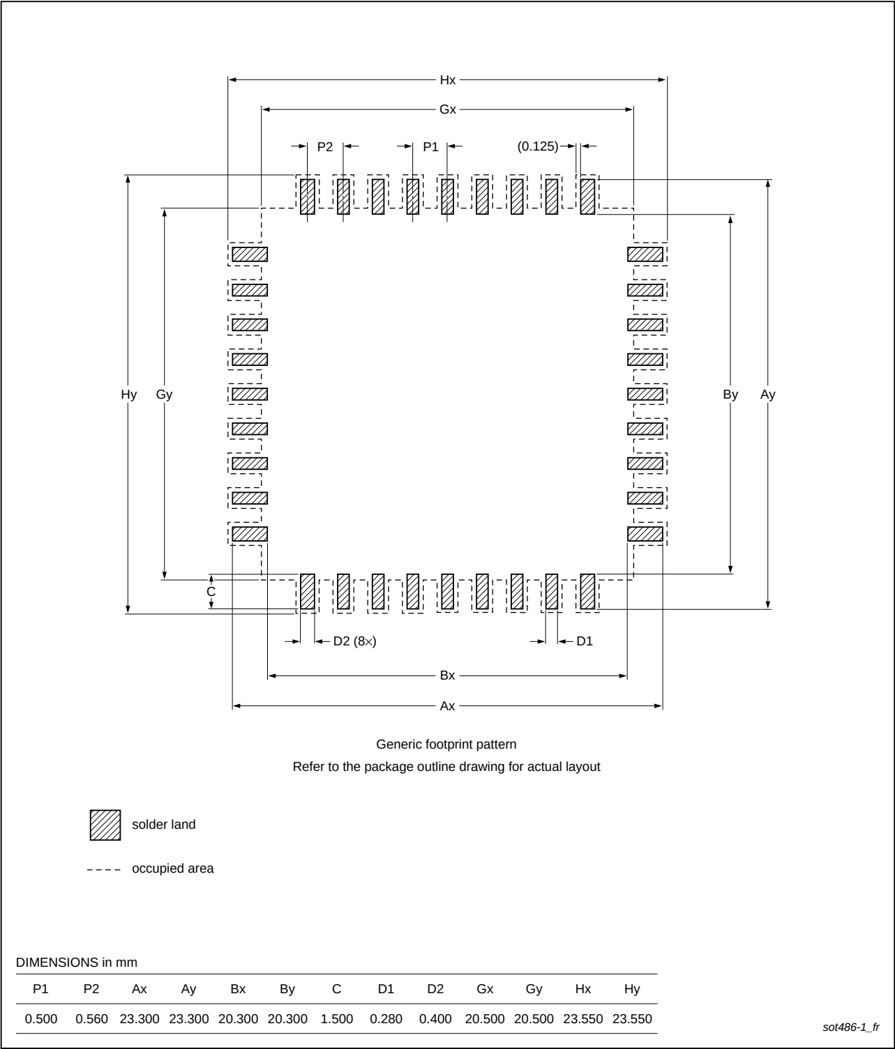
Footprint information for reflow soldering of LQFP144 package SOT486-1
