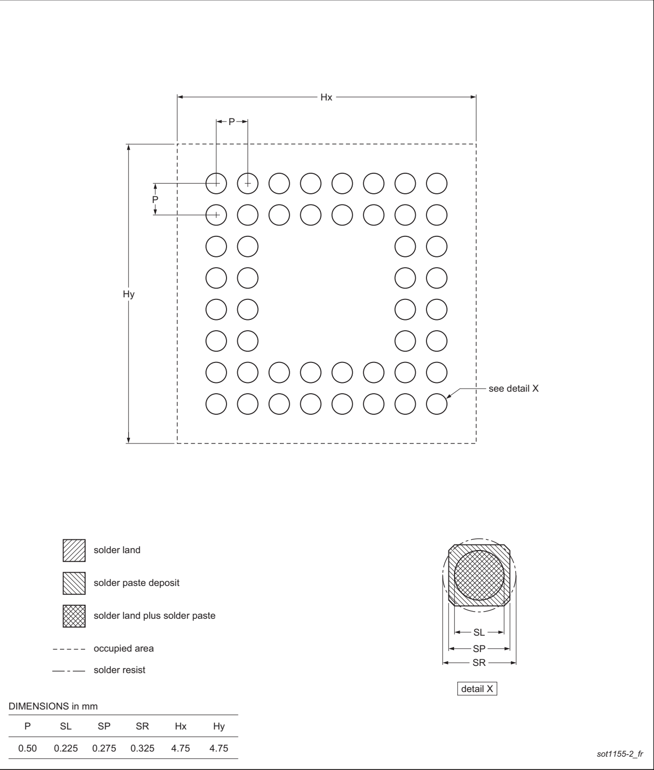
Fig 41. Reflow soldering for the TFBGA48 package
