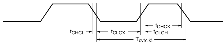
Fig 21. External clock timing (with an amplitude of at least V_{i(RMS)} = 200 mV)
