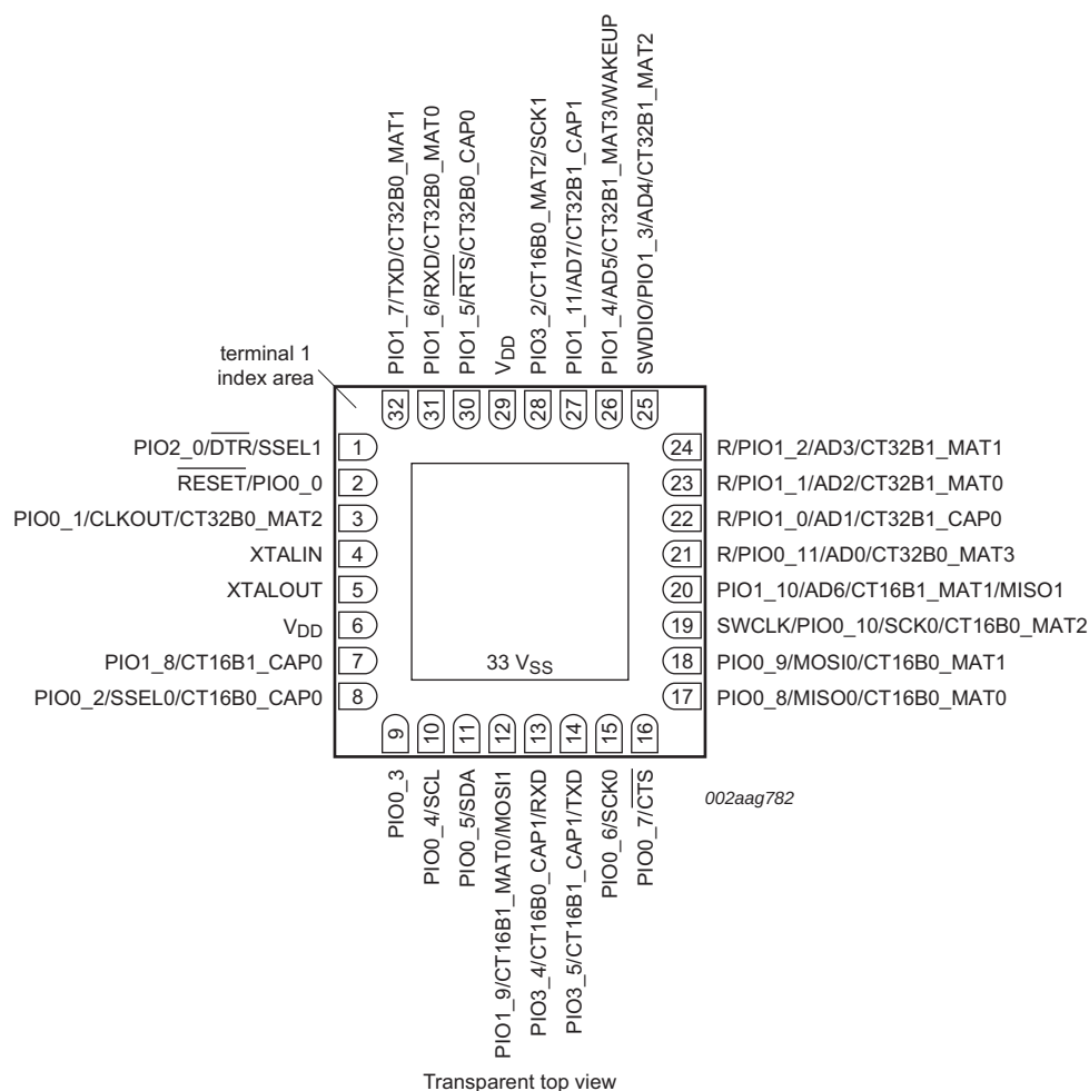
Fig 7. LPC1100XL series pin configuration HVQFN33
