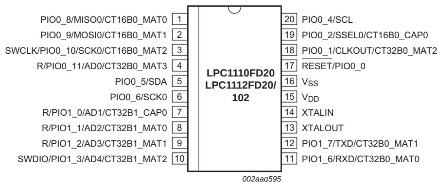
Fig 8. LPC1100L series pin configuration SO20 package
