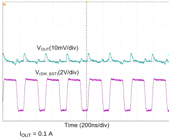
Figure 107. Boost Output Voltage Ripple
