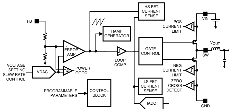
Figure 7. Detailed Block Diagram Showing One Buck Converter
