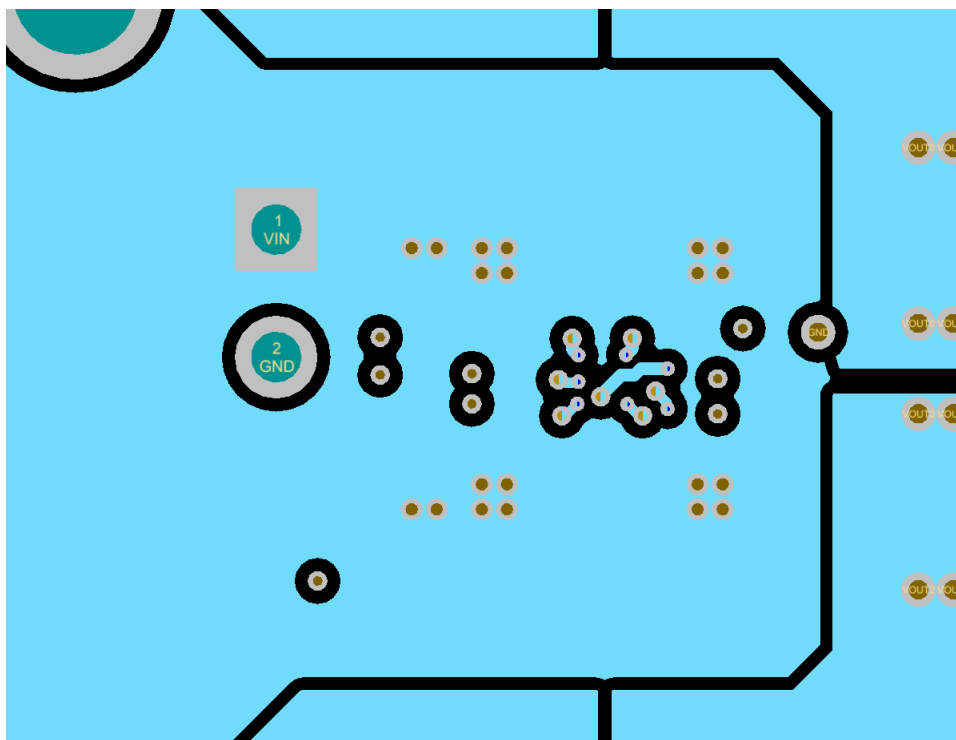
Figure 9. Third Layer (VIN)
