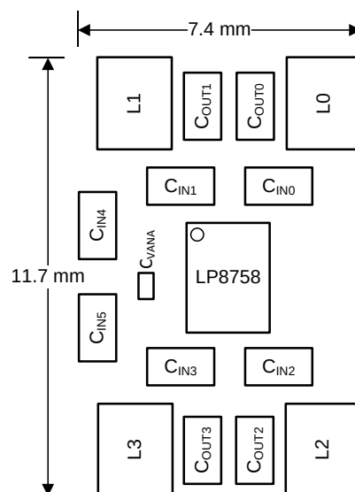
Figure 6. Component Placement near the LP8758 Device
