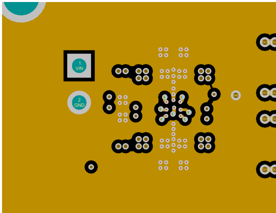
Figure 8. Second Layer (GND)
