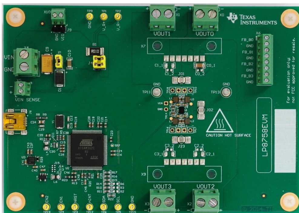
Figure 1. LP8758EVM
