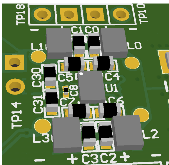
Figure 11. 3D view Showing the LP8758 Device and Nearest Components
