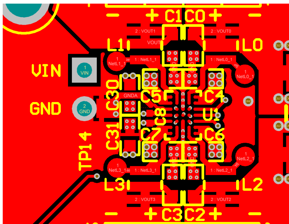
Figure 6. Component Placement near the LP8758 Device
