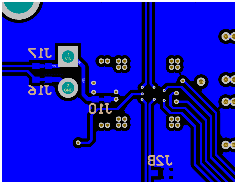
Figure 10. Bottom Layer and Silk
