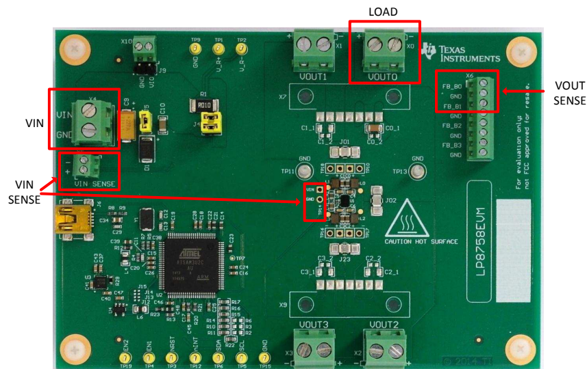
Figure 4. Connections for Efficiency Measurement
