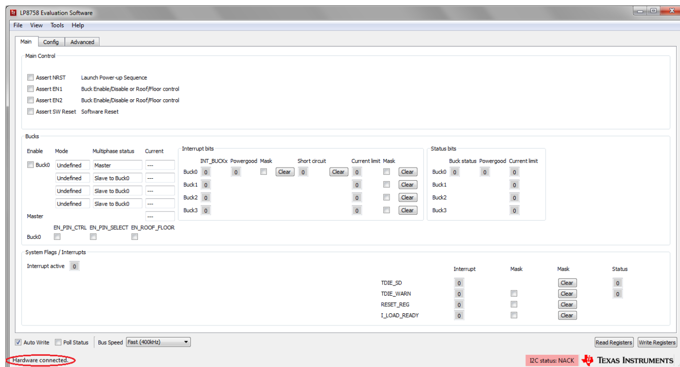
Figure 2. Evaluation Software Graphical User Interface (GUI) When Board Connected
