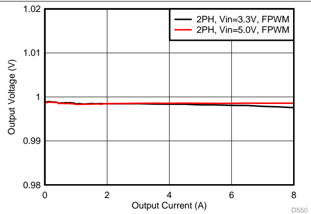
Figure 48. Output Voltage vs Load Current in Forced-PWM Mode (2-Phase Output)
