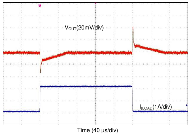
Figure 81. Transient from PWM-to-PFM Mode (1-Phase Output)
