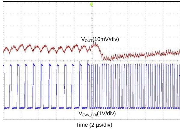
Figure 34. Transient from PFM-to-PWM Mode (1-Phase Output)
