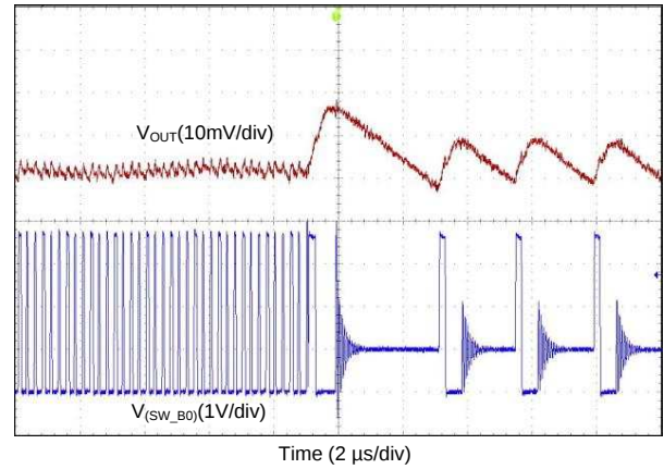
Figure 35. Transient from PWM-to-PFM Mode (1-Phase Output)
