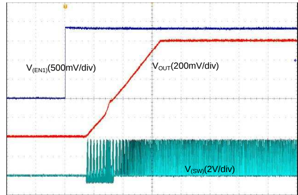
Figure 29. Start-Up With EN1, Forced PWM
