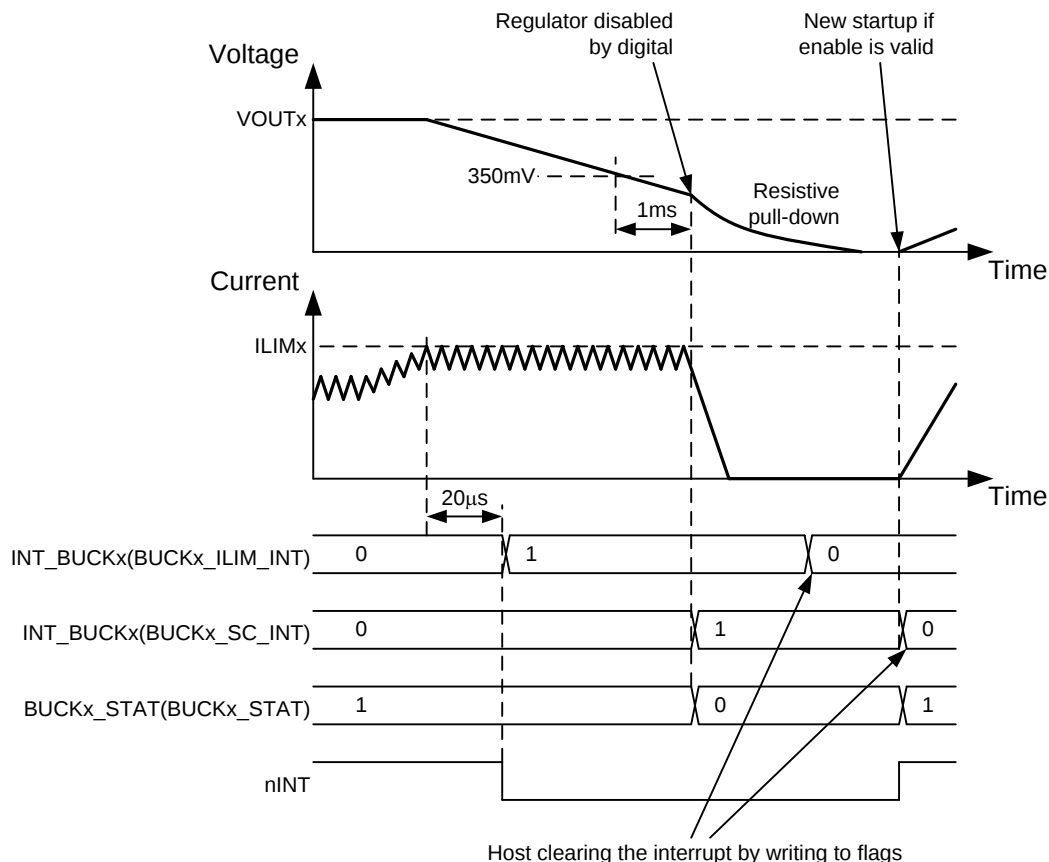
Figure 13. Overload Situation
