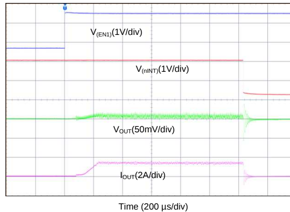
Figure 40. Start-up With Short on Output (1-Phase Output)
