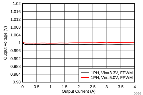
Figure 25. Output Voltage vs Load Current in Forced-PWM Mode
