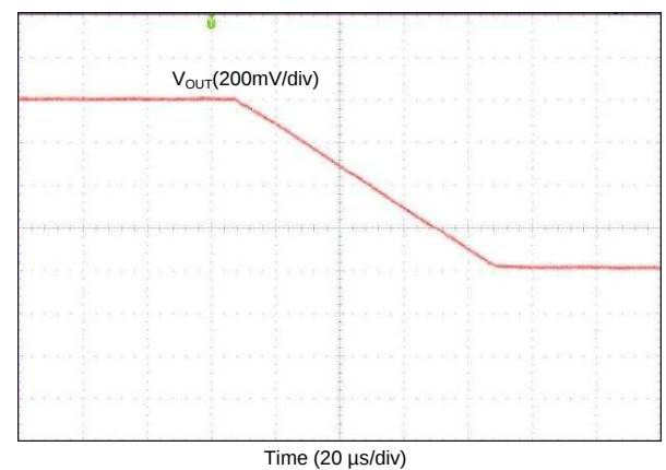
Figure 37. Transient Load Step Response, Forced-PWM Mode (1-Phase Output)
