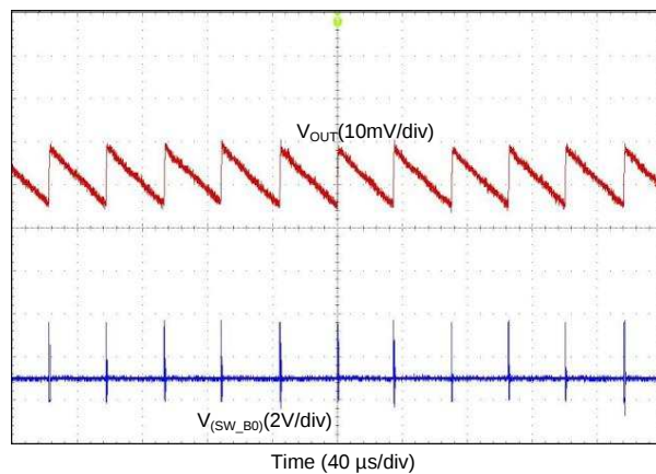
Figure 32. Output Voltage Ripple, PFM Mode (1-Phase Output)
