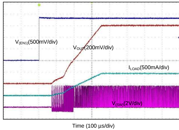
Figure 30. Start-Up With EN1, Forced PWM (1-Phase Output)
