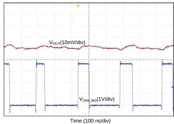
Figure 33. Output Voltage Ripple, Forced-PWM Mode (1-Phase Output)
