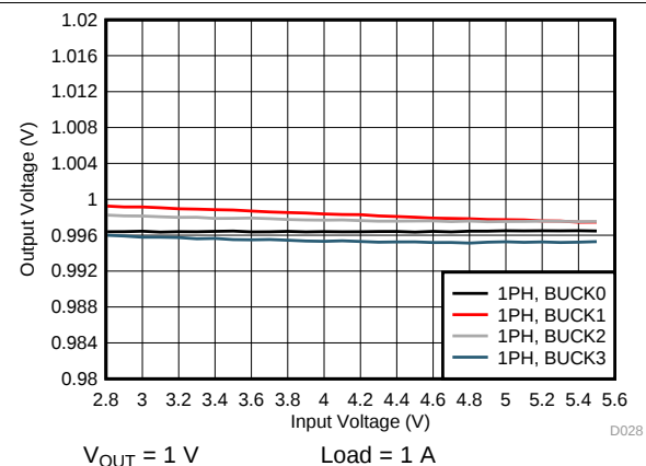
Figure 27. Output Voltage vs Input Voltage in PWM Mode
