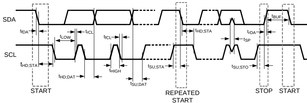
Figure 17. I²C-Compatible Timing
