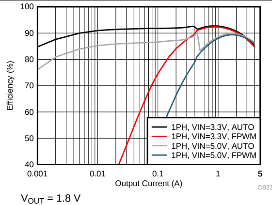
Figure 22. Efficiency in PFM/PWM Mode
