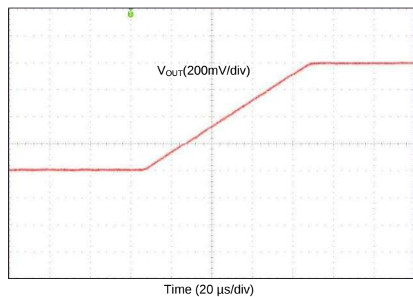
Figure 38. V_{OUT} Transition from 0.6 V to 1.4 V
