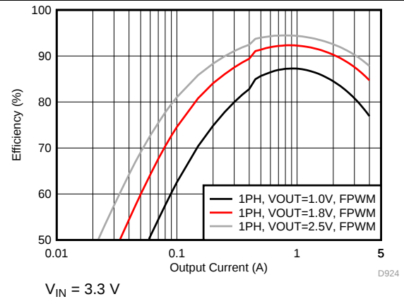
Figure 23. Efficiency in Forced-PWM Mode
