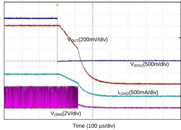
Figure 31. Shutdown With EN1, Forced PWM (1-Phase Output)
