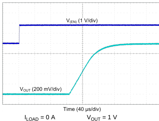
Figure 112. LDO Start-Up
