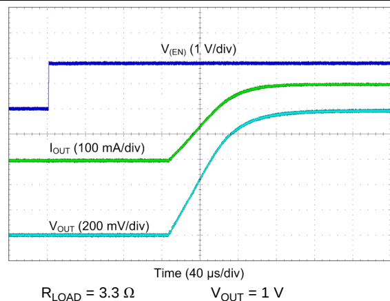
Figure 113. LDO Start-Up
