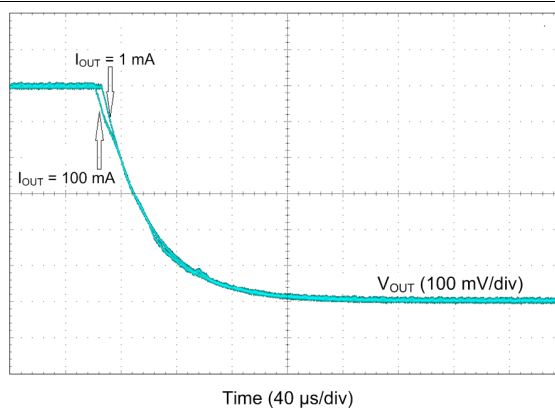
Figure 114. LDO Shutdown
