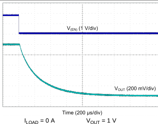
Figure 114. LDO Shutdown
