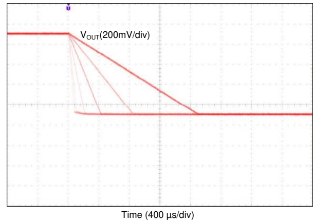
Figure 106. Buck V_{OUT} Transition from 1.4 V to 0.6 V With Different Slew Rate Settings
