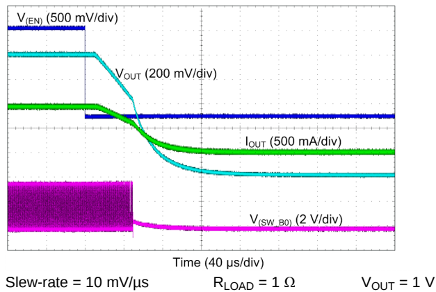
Figure 89. Buck Shutdown With EN1, Forced PWM Mode (Single-Phase Output)
