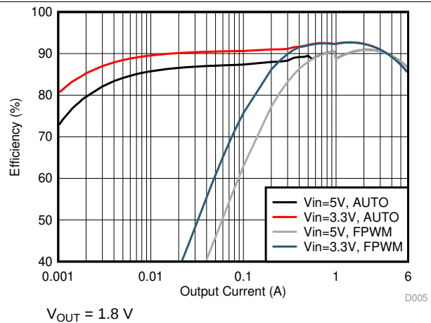
Figure 72. Buck Efficiency in PFM/PWM and Forced PWM Mode (Dual-Phase Output)
