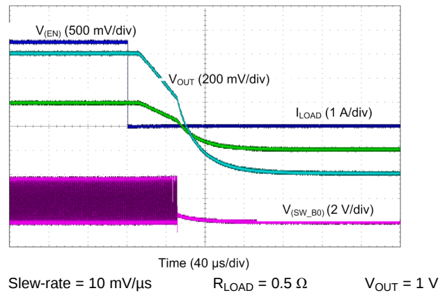
Figure 90. Buck Shutdown With EN1, Forced PWM Mode (Dual-Phase Output)
