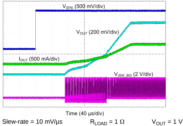
Figure 87. Buck Start-Up with EN1, Forced PWM Mode (Single-Phase Output)
