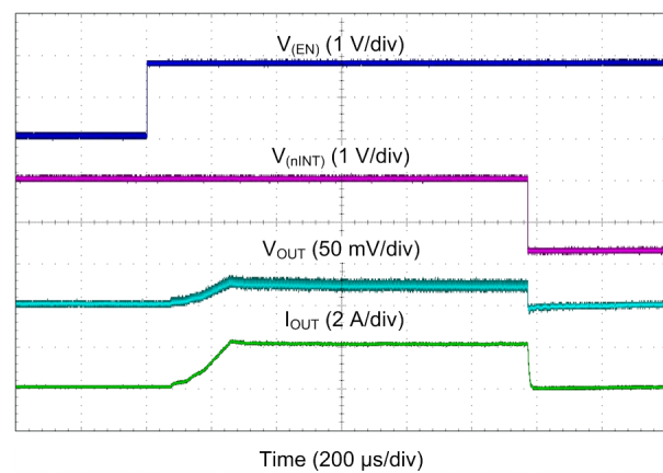
Figure 108. Buck Start-up With Short on Output (Dual-Phase Output)
