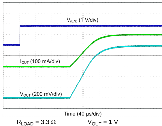
Figure 113. LDO Start-Up
