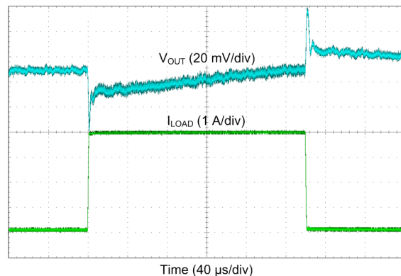
Figure 102. Buck Transient Load Step Response, AUTO Mode (Dual-Phase Output)
