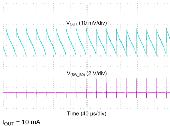
Figure 91. Buck Output Voltage Ripple, PFM Mode (Single-Phase Output)
