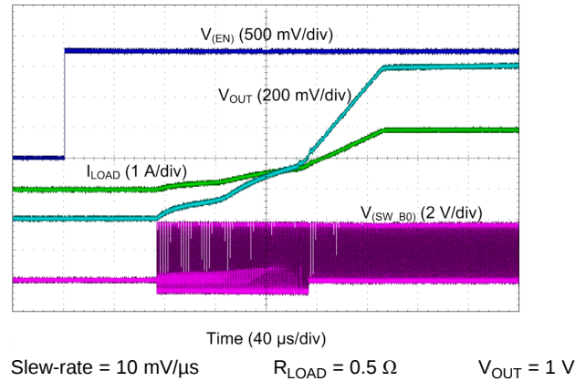
Figure 88. Buck Start-Up with EN1, Forced PWM Mode (Dual-Phase Output)
