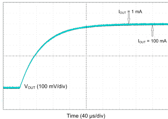
Figure 117. LDO V_{OUT} Transition from 1.2 V to 1.8 V
