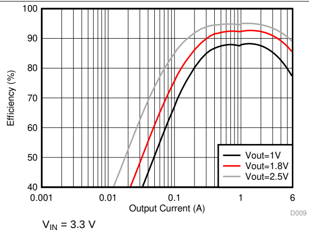
Figure 74. Buck Efficiency in Forced PWM Mode (Dual-Phase Output)
