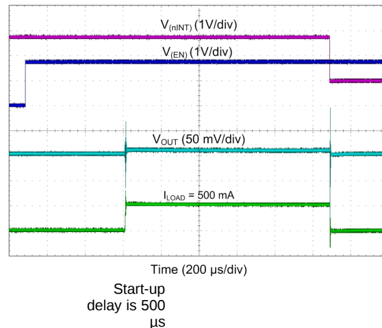
Figure 118. LDO Start-Up With Short on Output
