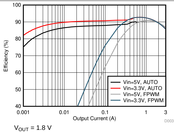
Figure 71. Buck Efficiency in PFM/PWM and Forced PWM Mode (Single-Phase Output)
