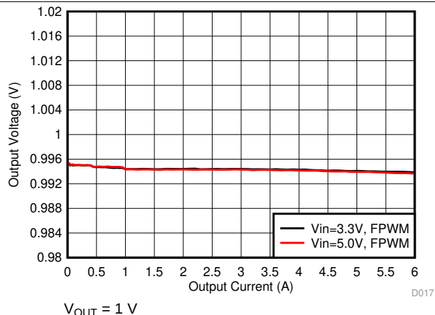
Figure 78. Buck Output Voltage vs Load Current in Forced PWM Mode (Dual-Phase Output)
