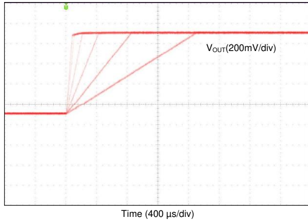
Figure 105. Buck V_{OUT} Transition from 0.6 V to 1.4 V With Different Slew Rate Settings
