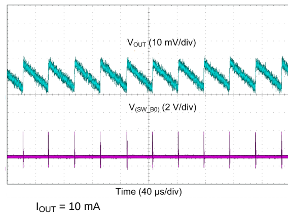
Figure 92. Buck Output Voltage Ripple, PFM Mode (Dual-Phase Output)
