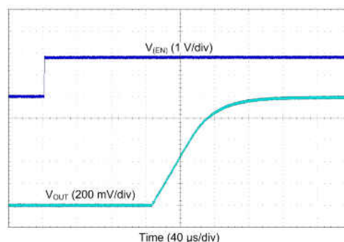
Figure 8-45. LDO Start-Up
