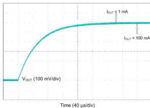
Figure 8-50. LDO V_{OUT} Transition from 1.2 V to 1.8 V
