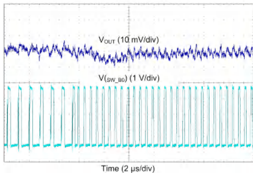
Figure 8-28. Buck Transient From PFM-to-PWM Mode (Single-Phase Output)
