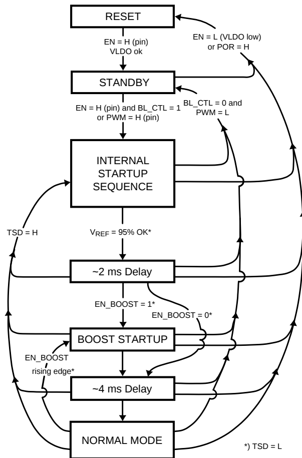
Figure 19. Device Functional Modes
