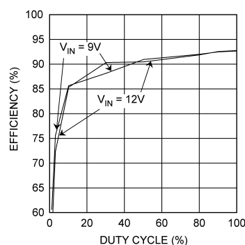
LED Drive Efficiency
