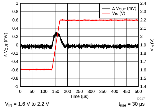
Figure 26. LP5912-0.9 Line Transient
