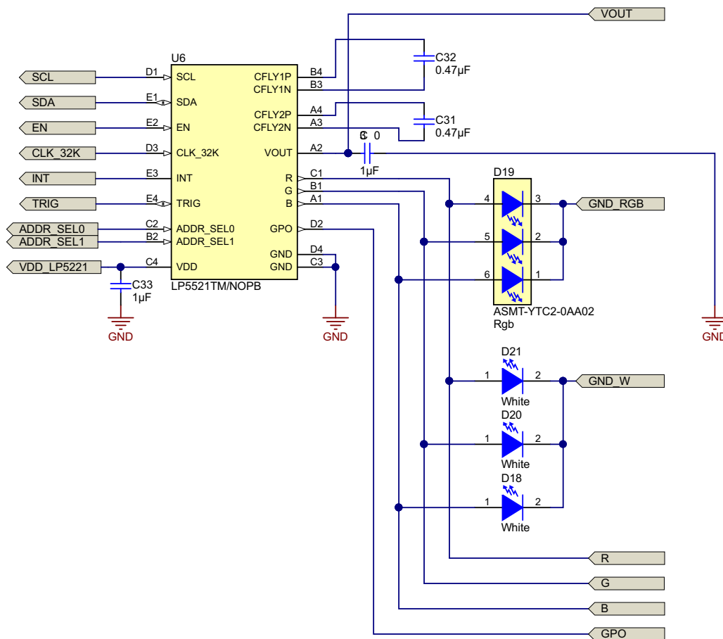
Figure 7. LP5521 (Device 1)
