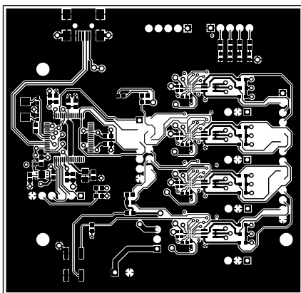
Figure 12. Layer 1 (Top, Signal)
