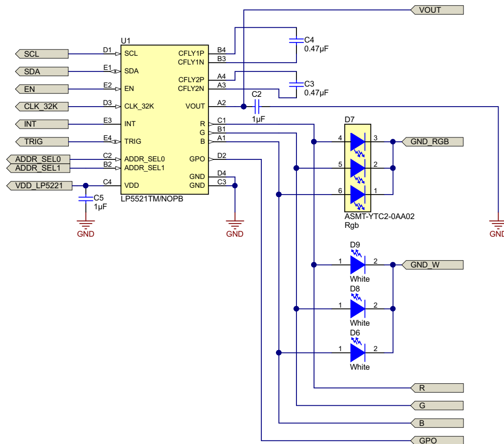
Figure 10. LP5521 (Device 4)
