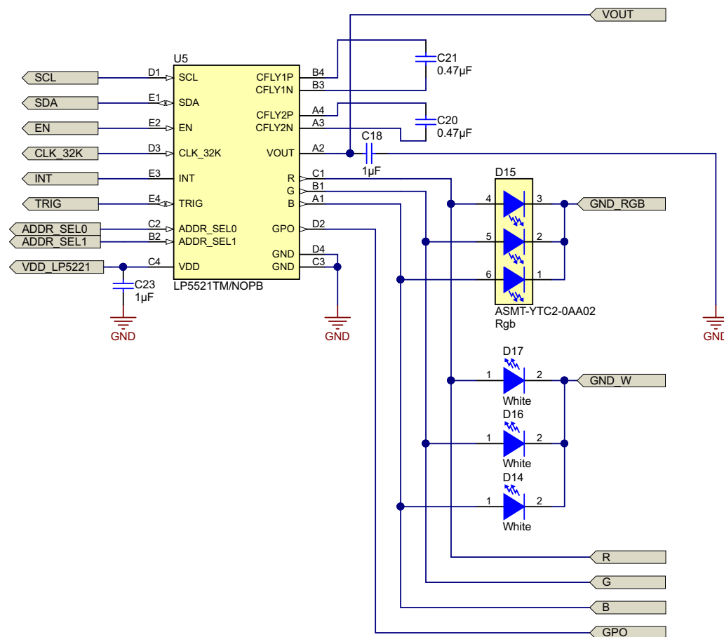
Figure 8. LP5521 (Device 2)
