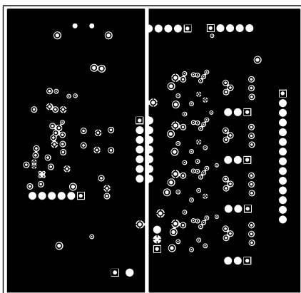
Figure 14. Layer 4 (Power)
