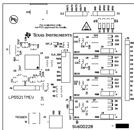
Figure 11. Top Overlay
