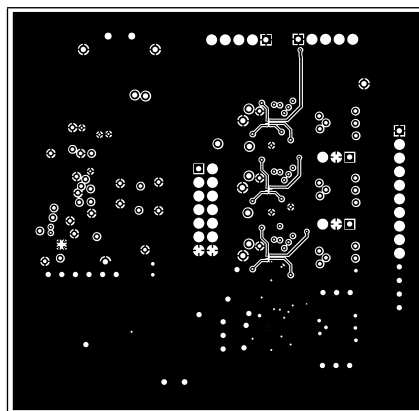
Figure 13. Layer 2 (GND)
