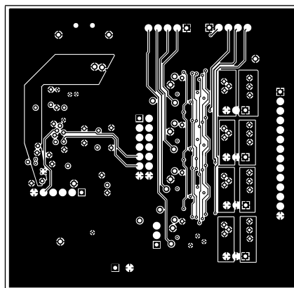
Figure 15. Layer 4 (Bottom, Signal)
