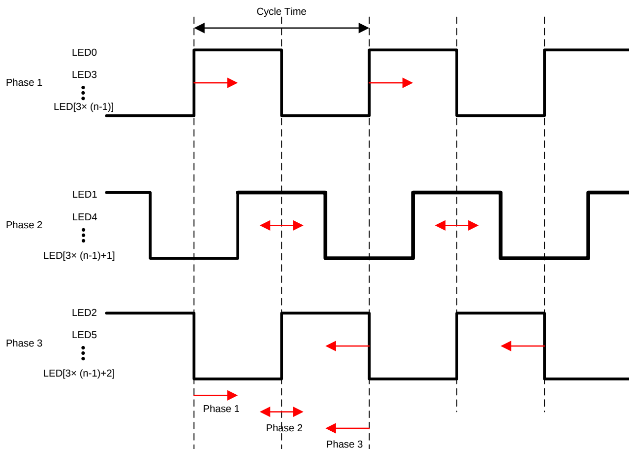
Figure 12. PWM Phase-Shifting
