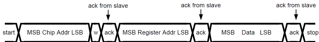
Figure 19. Write Cycle
