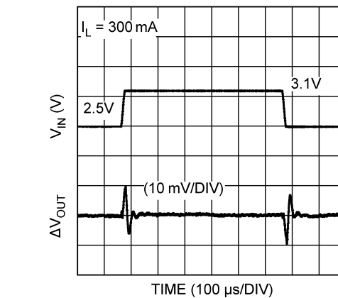
Figure 17. Line Transient
