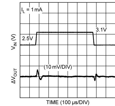
Figure 16. Line Transient
