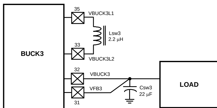
Figure 68. Schematic Section for Buck3 Operation
