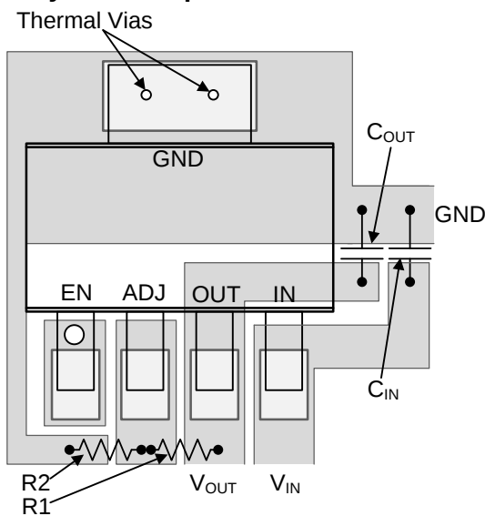
Figure 33. LP38692-ADJ SOT-223 Package
