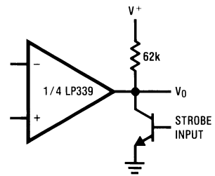
Output Strobing
