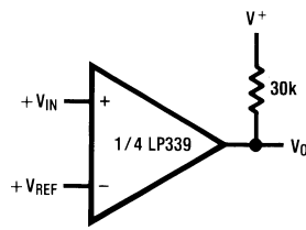
Basic Comparator
