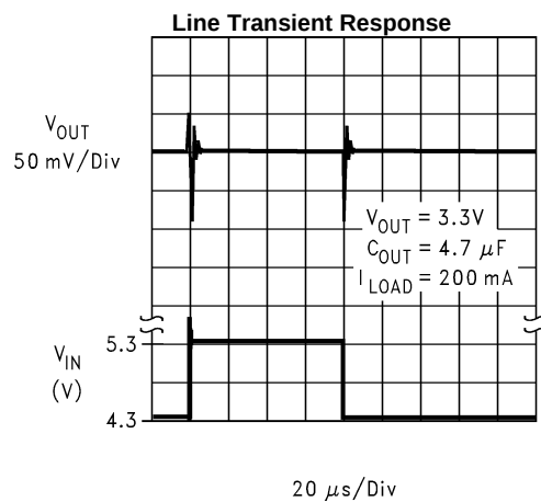
20 \mu\text{s}/\text{Div} Figure 16.
