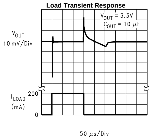
50 \mu\text{s}/\text{Div} Figure 14.
