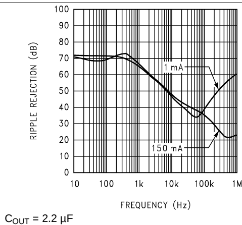
Figure 13. Ripple Rejection
