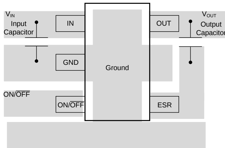
Figure 27. LP2983 Layout Example
