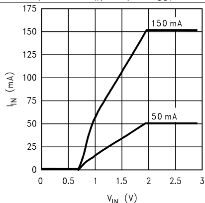
Figure 5. Input Current vs V_{IN}
