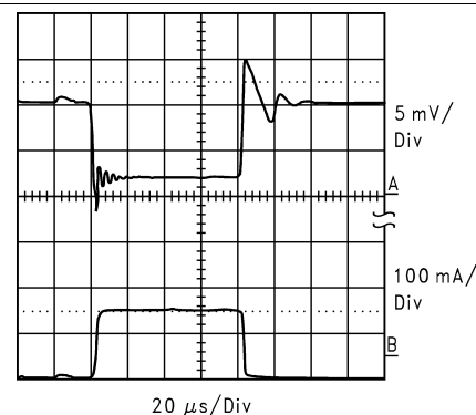
Figure 26. Load Transient Response
