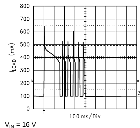
Figure 14. Turnon Time
