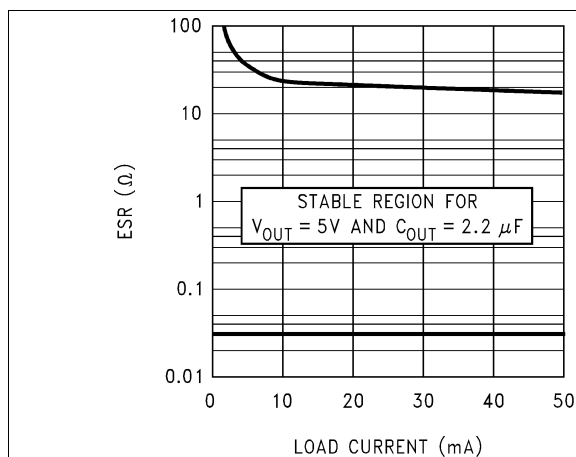
Figure 40. 5-V, 2.2-μF ESR Curves
