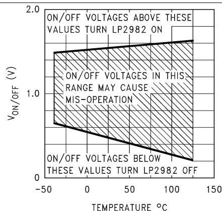
Figure 26. ON/OFF Threshold vs Temperature
