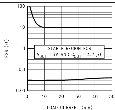
Figure 41. 3-V, 4.7-μF ESR Curves
