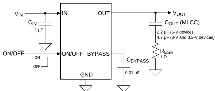
Figure 37. Typical Application With Ceramic C OUT Series R
