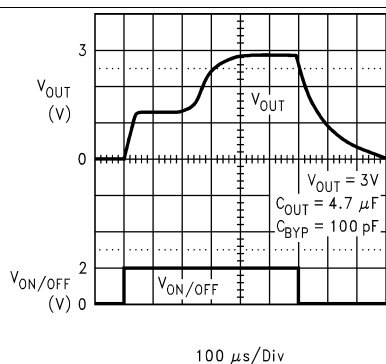
Figure 33. Turnon Waveform
