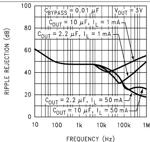
Figure 32. Ripple Rejection
