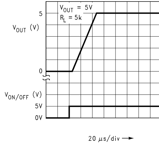
Figure 28. Turnon Waveform
