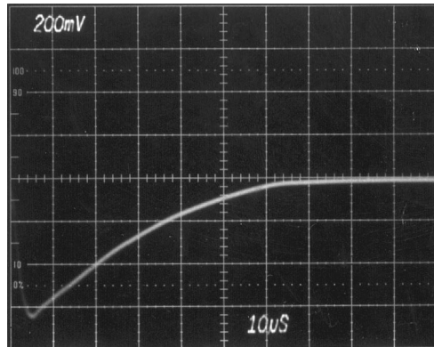
Transient Response for 0–0.5A Load Step
