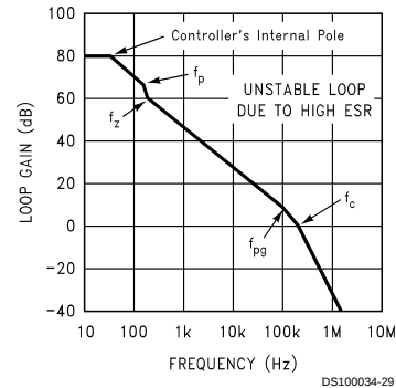
High ESR Unstable without Feed-Forward
