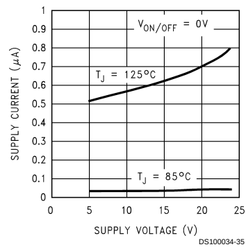
Leakage Current
