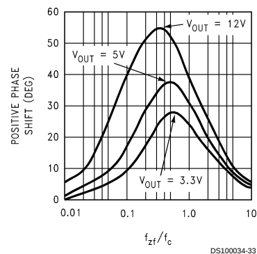
Phase Lead Provided by C_F
