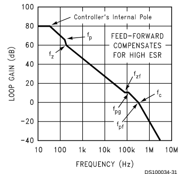
High ESR Corrected with Feed-Forward
