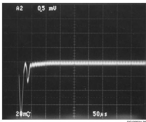
Transient Response with Output Capacitor Halved
