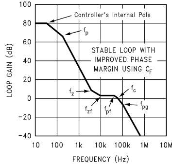
Improved Phase Margin with Feed-Forward
