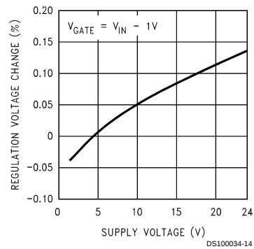
Line Regulation
