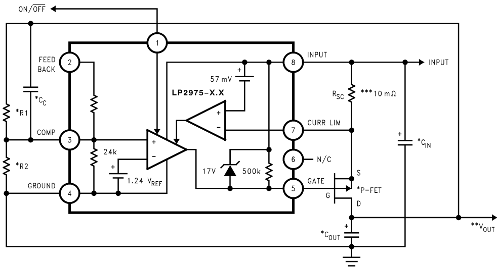
Adjustable Voltage 5A LDO Regulator
