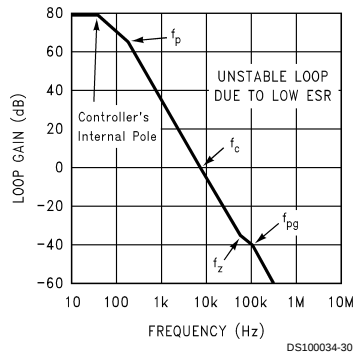
Low ESR Unstable without Feed-Forward
