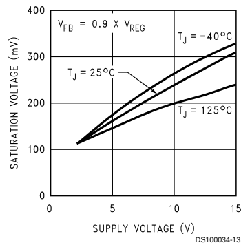
Gate-Ground Saturation
