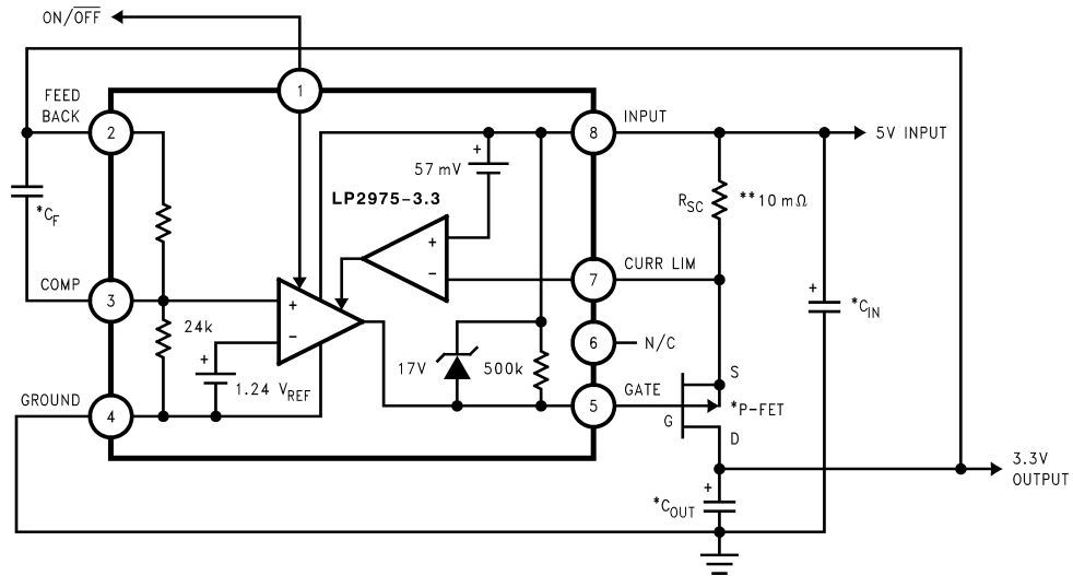
5V - 3.3V @ 5A LDO Regulator
