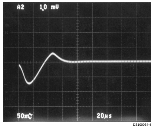
Transient Response for 0–6A Load Step
