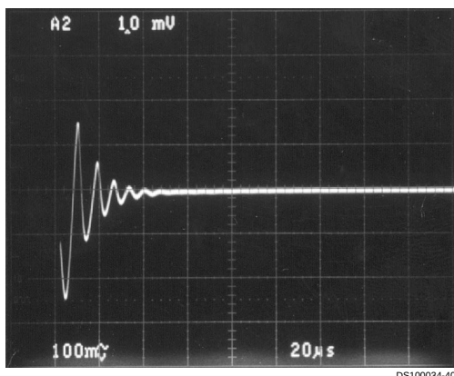
Transient Response with Only 4.7 μF Output Cap
