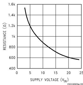
Gate Pin Output Impedance
