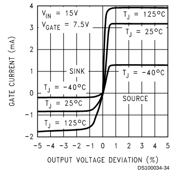
Gate Current
