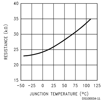
ON/OFF Input Resistance
