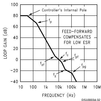
Low ESR Corrected with Feed-Forward
