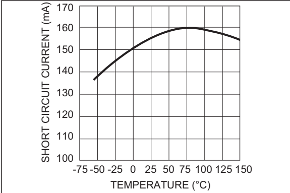
FIGURE 2-10: Short Circuit Current.
