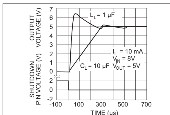
FIGURE 2-21: Enable Transient.
