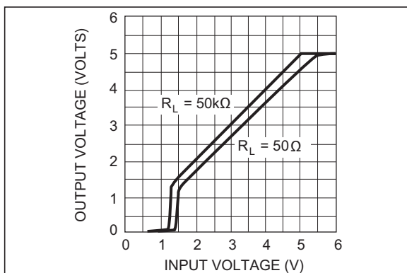
FIGURE 2-2: Dropout Characteristics.
