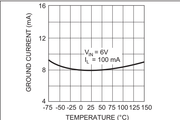
FIGURE 2-8: Ground Current.
