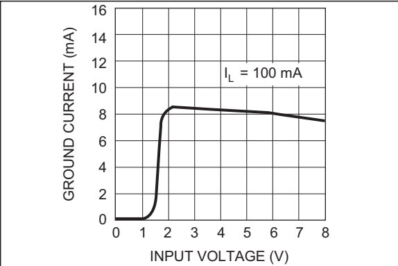
FIGURE 2-9: Ground Current.
