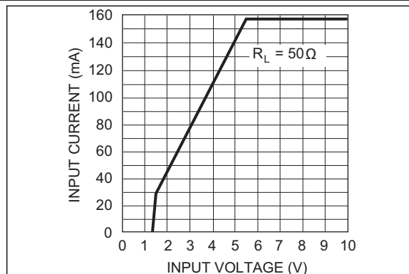
FIGURE 2-4: Input Current.
