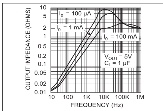
FIGURE 2-22: Output Impedance.
