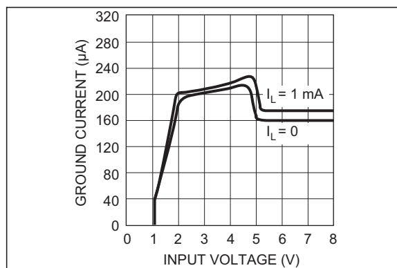
FIGURE 2-6: Ground Current.
