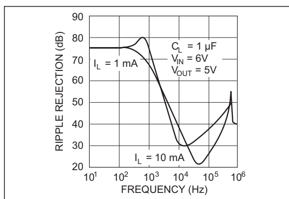
FIGURE 2-24: Ripple Rejection.
