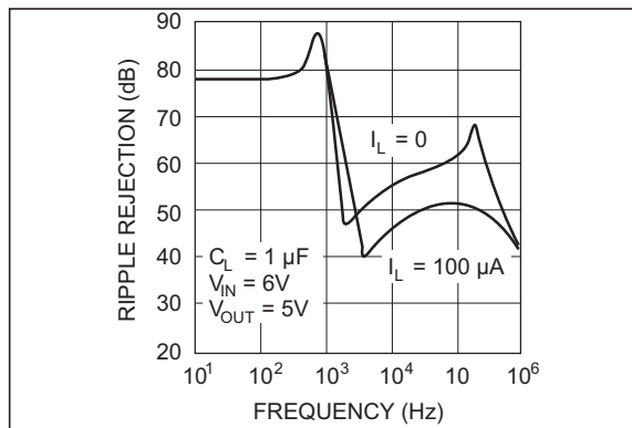
FIGURE 2-23: Ripple Rejection.
