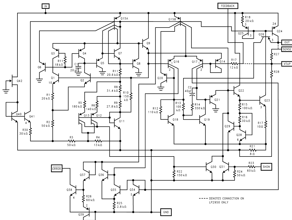
Figure 35. Schematic Diagram
