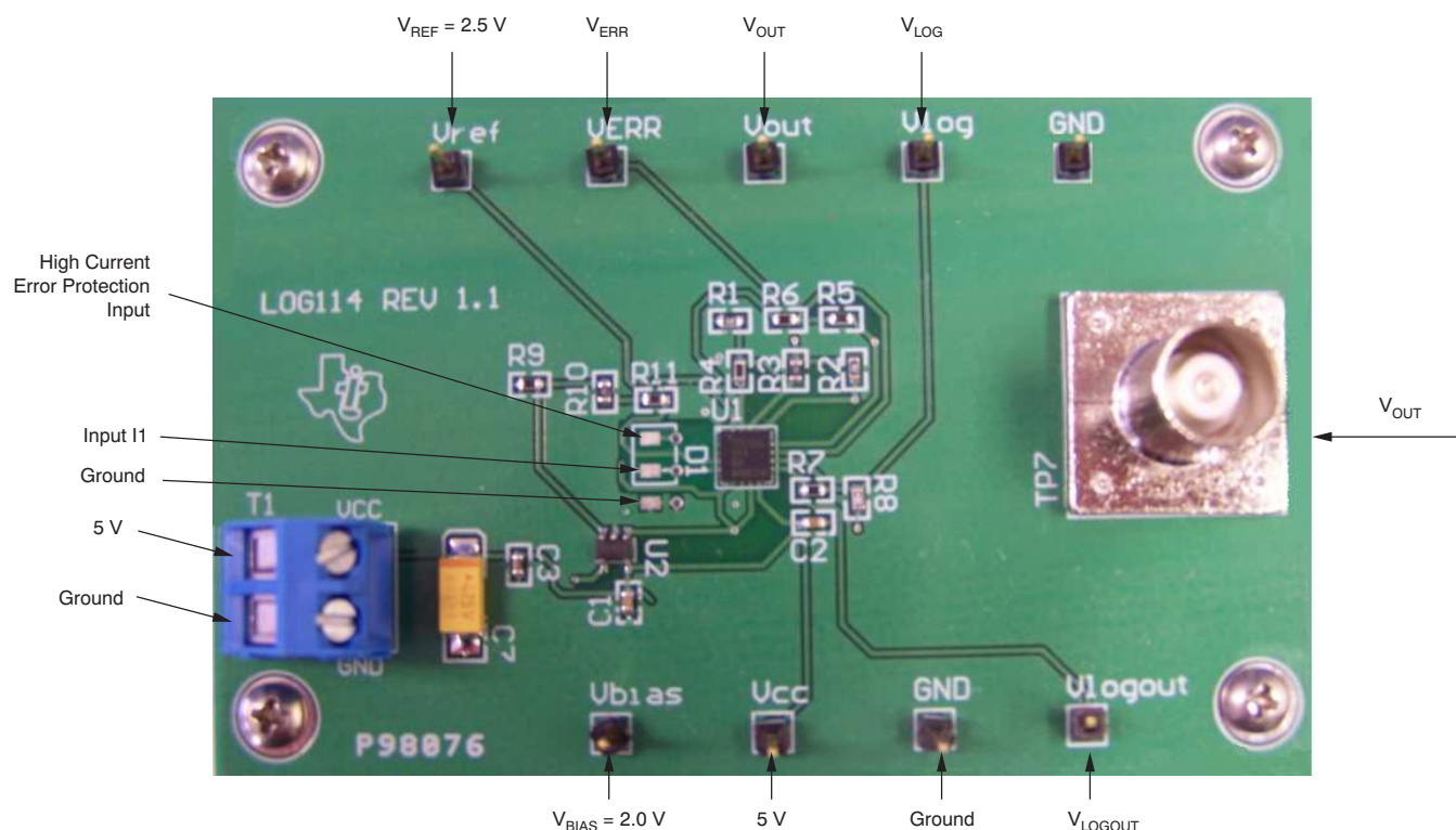
Figure 12. LOG114EVM Components
