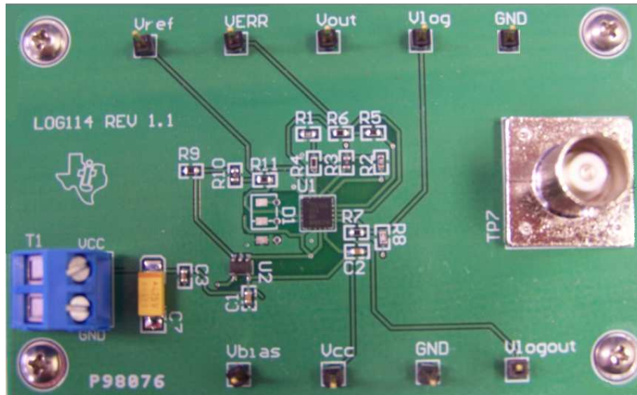
Figure 1. LOG114EVM
