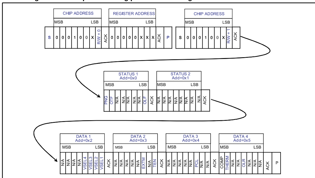
Figure 11: Example of reading procedure starting with first status address 0X0
