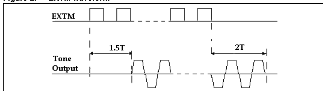
Figure 2. EXTM waveform
