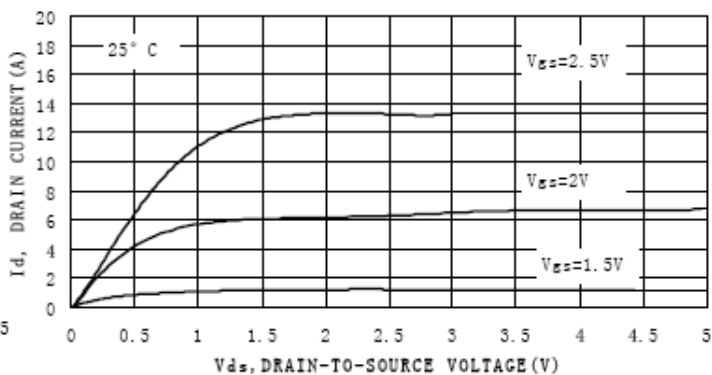
Figure 2. On-Region Characteristics
